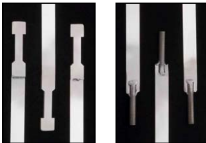
Close Up of Tension Strap Notched End and Threaded End
